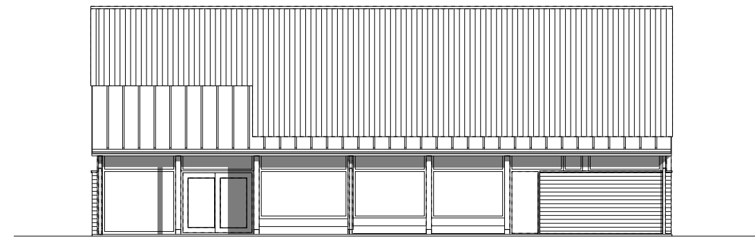
EAST FACADE
