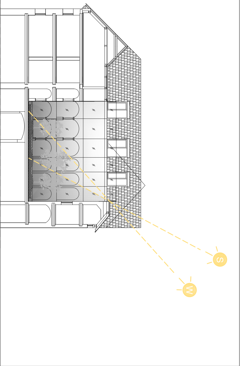
SECTION C-C
