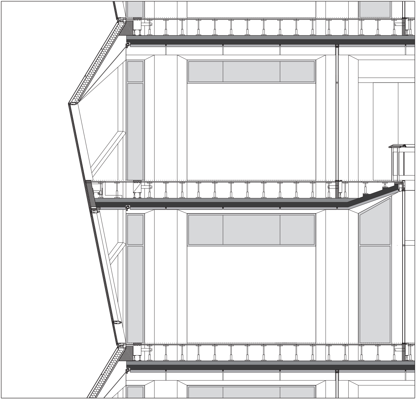
02 Detailed Section
