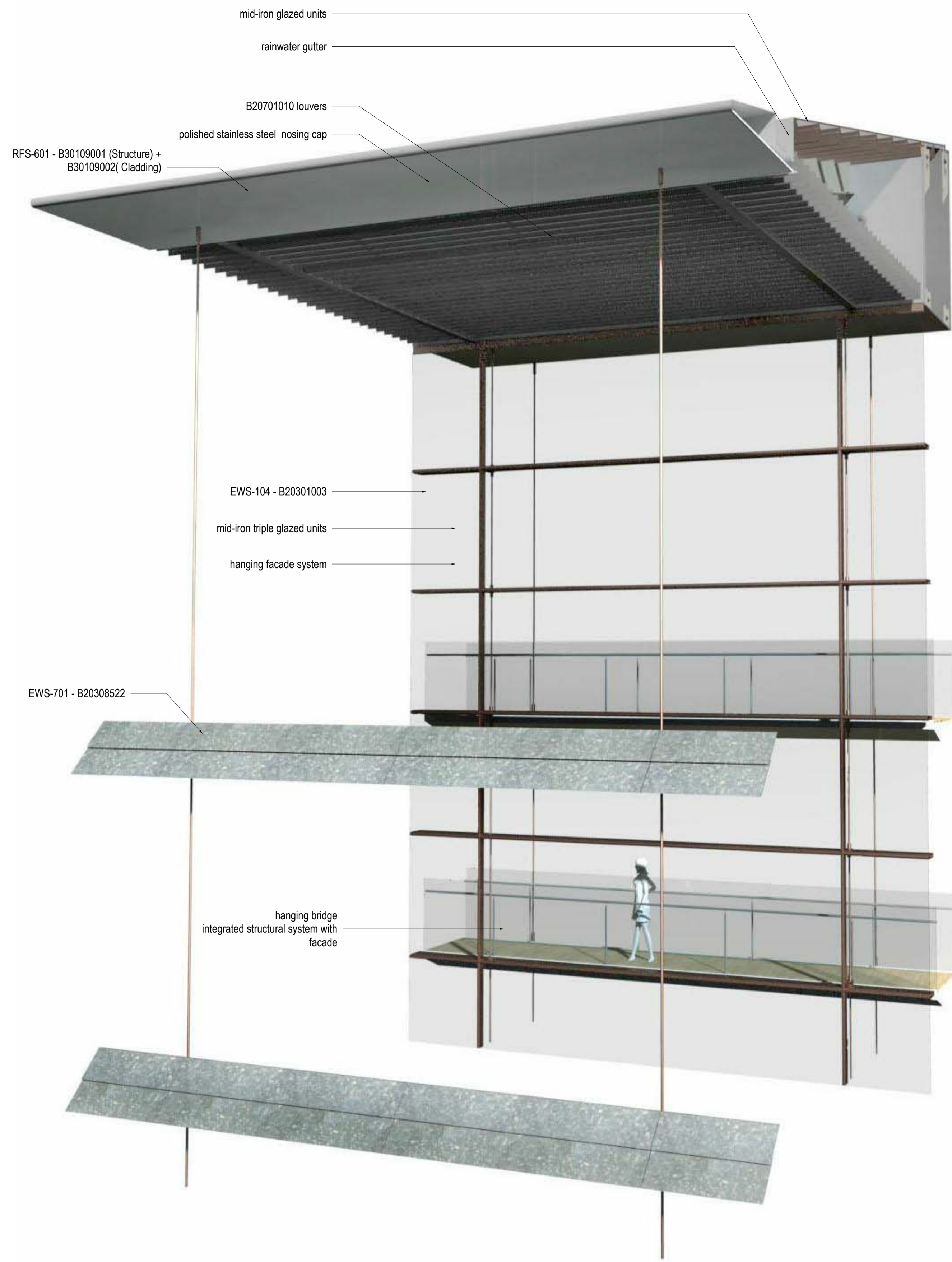
01 Sectional Perspective - Atrium Cladding NTS @ A1
