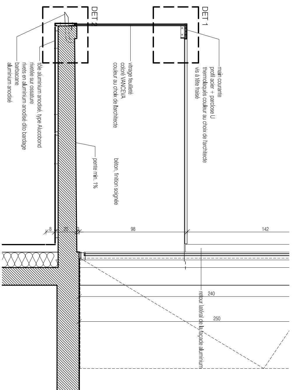
COUPE VERTICAL - BALCON 3M X 2M
