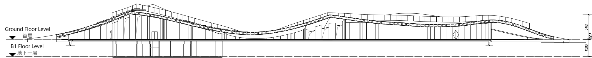
Section 1-1
