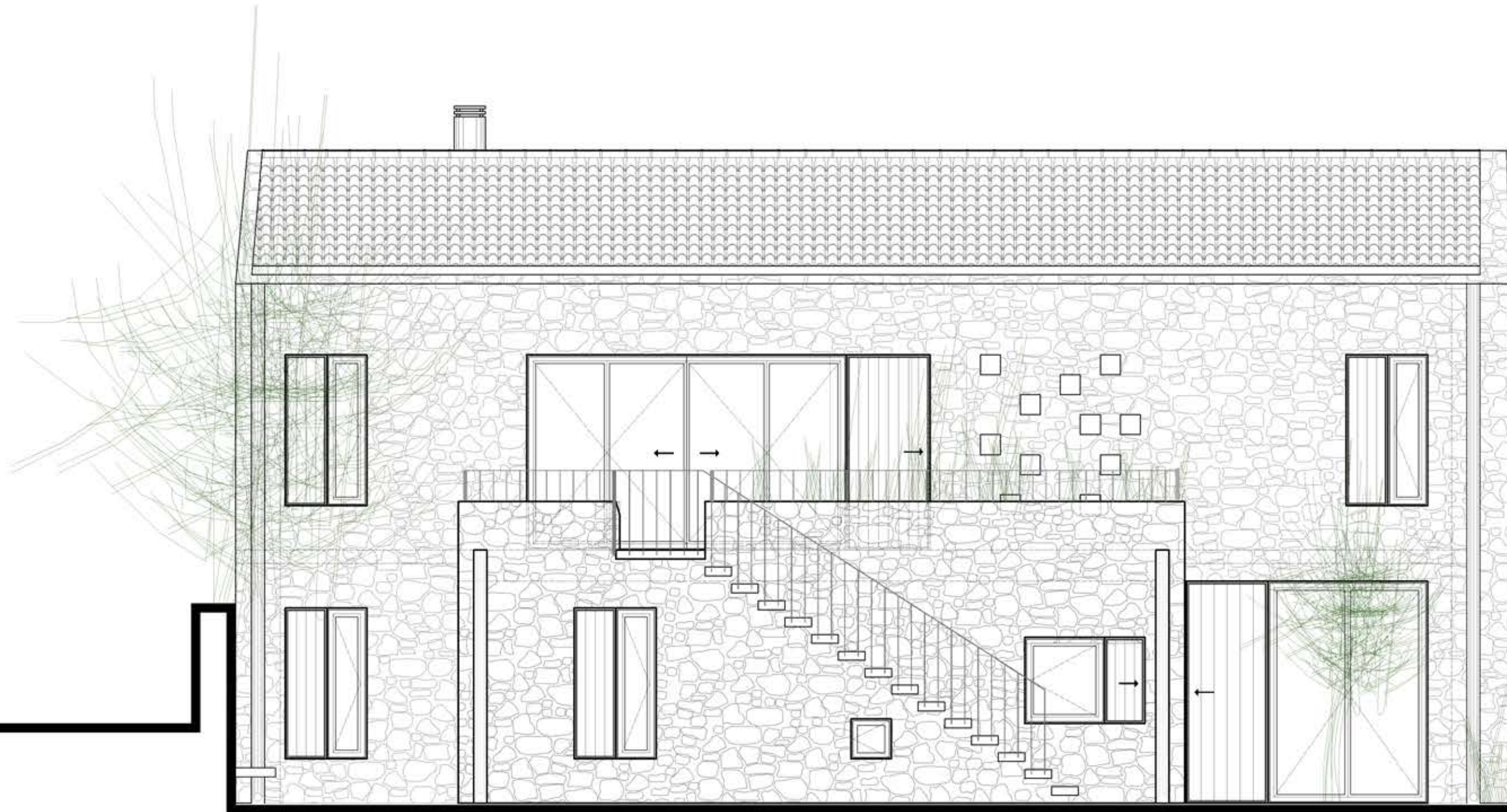
NORTH-EAST ELEVATION
