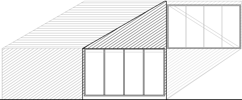
ELEVATION NORTH 0 50 100
