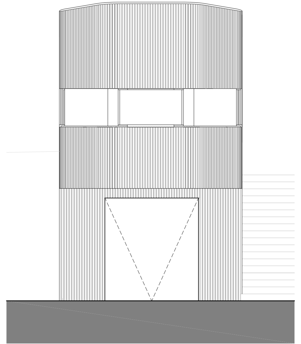
SOUTH ELEVATION
