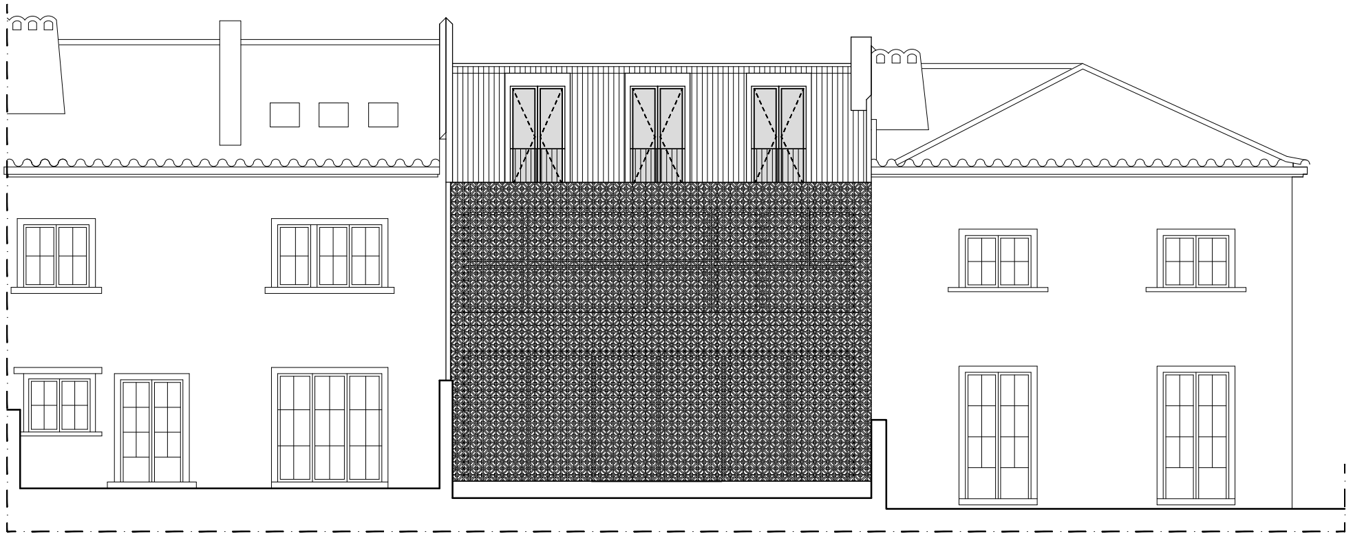
REAR ELEVATION
