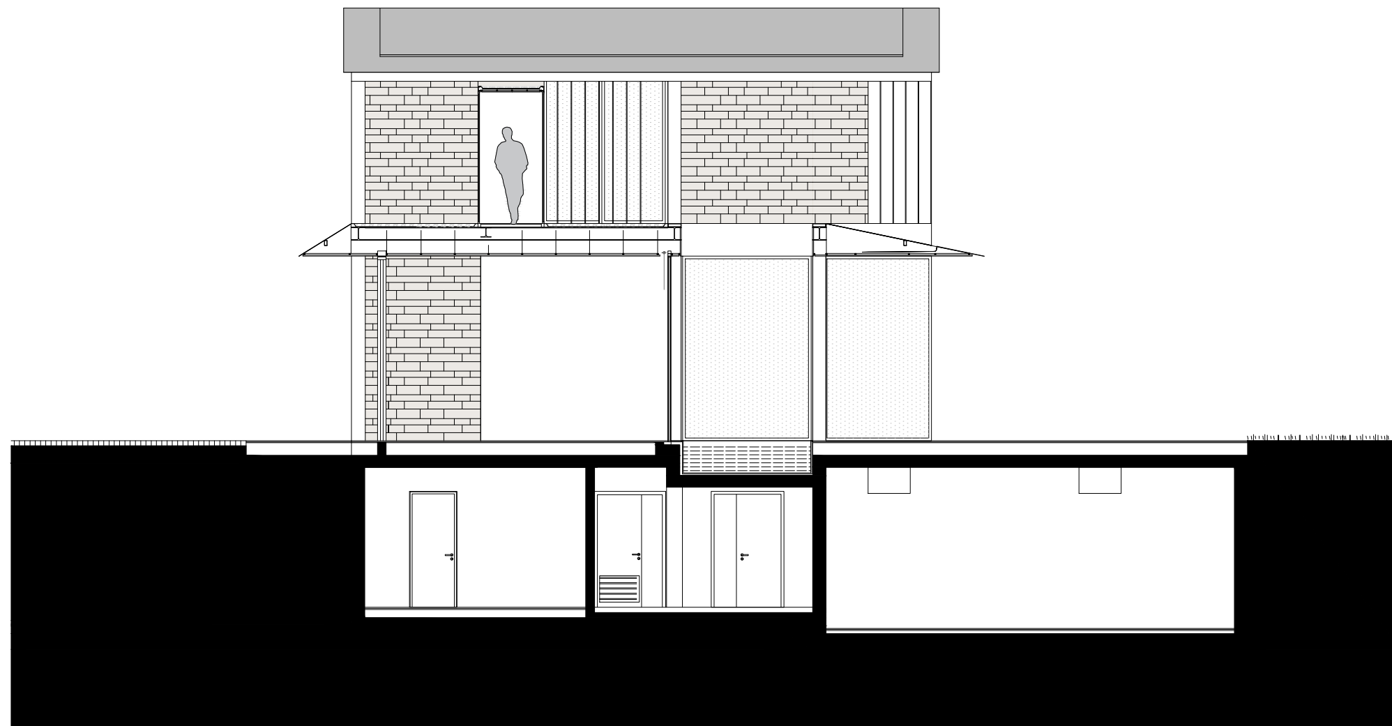
SECTION BB
