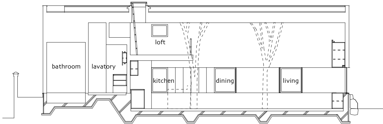
Section 02
