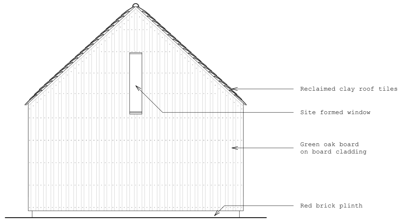
SOUTH EAST ELEVATION 1:50 @ A3
