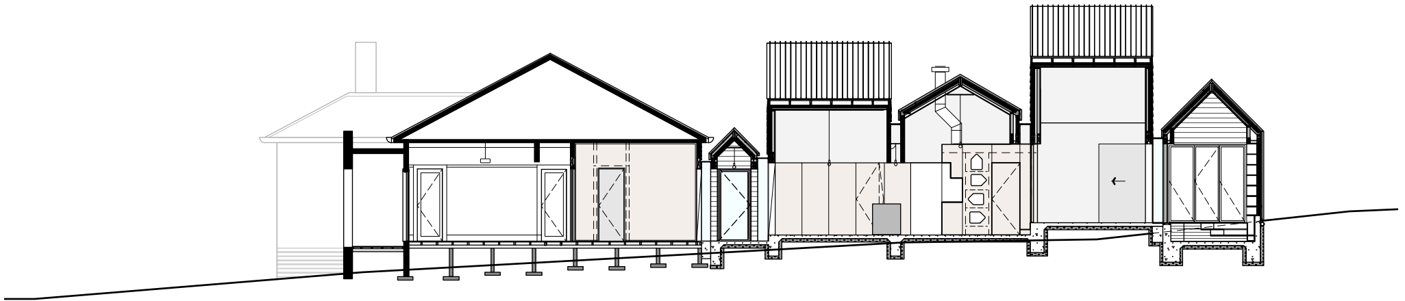
long section
