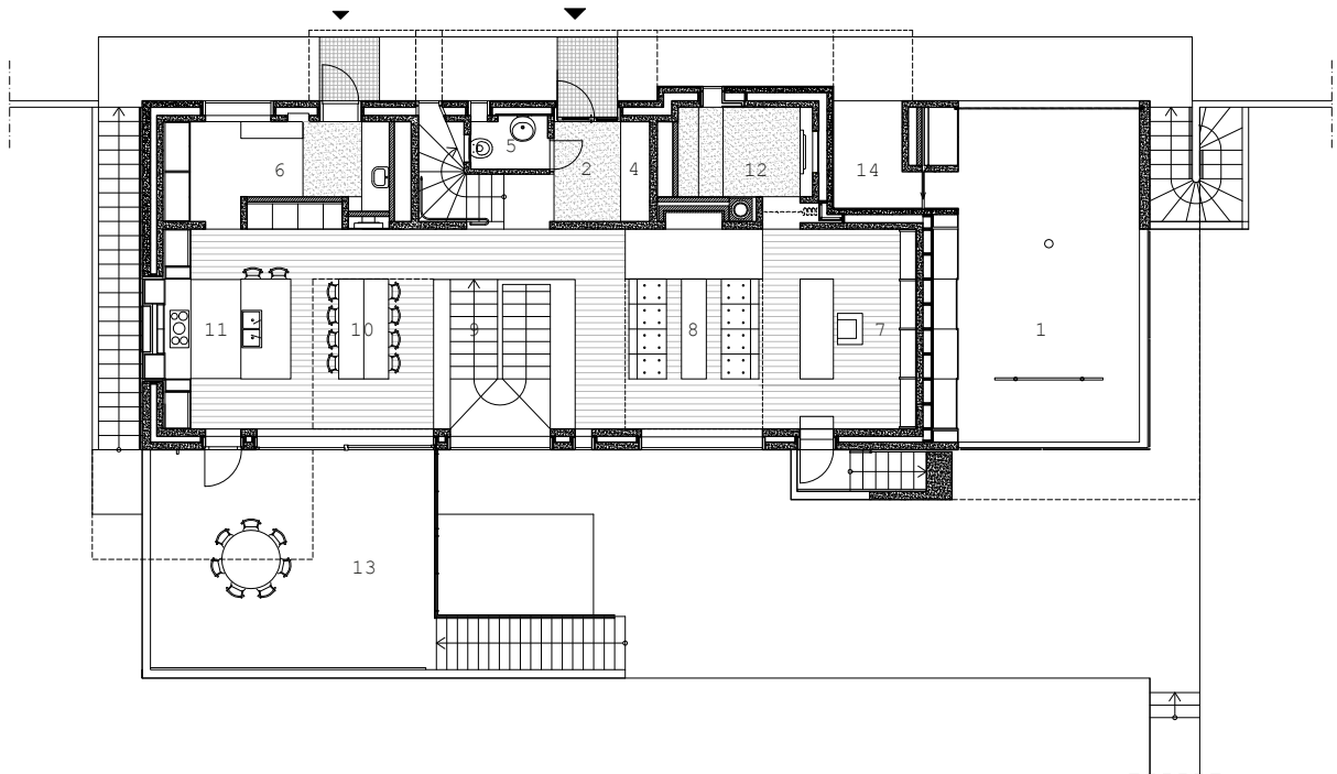
1ST FLOOR PLAN 1:200/A4
