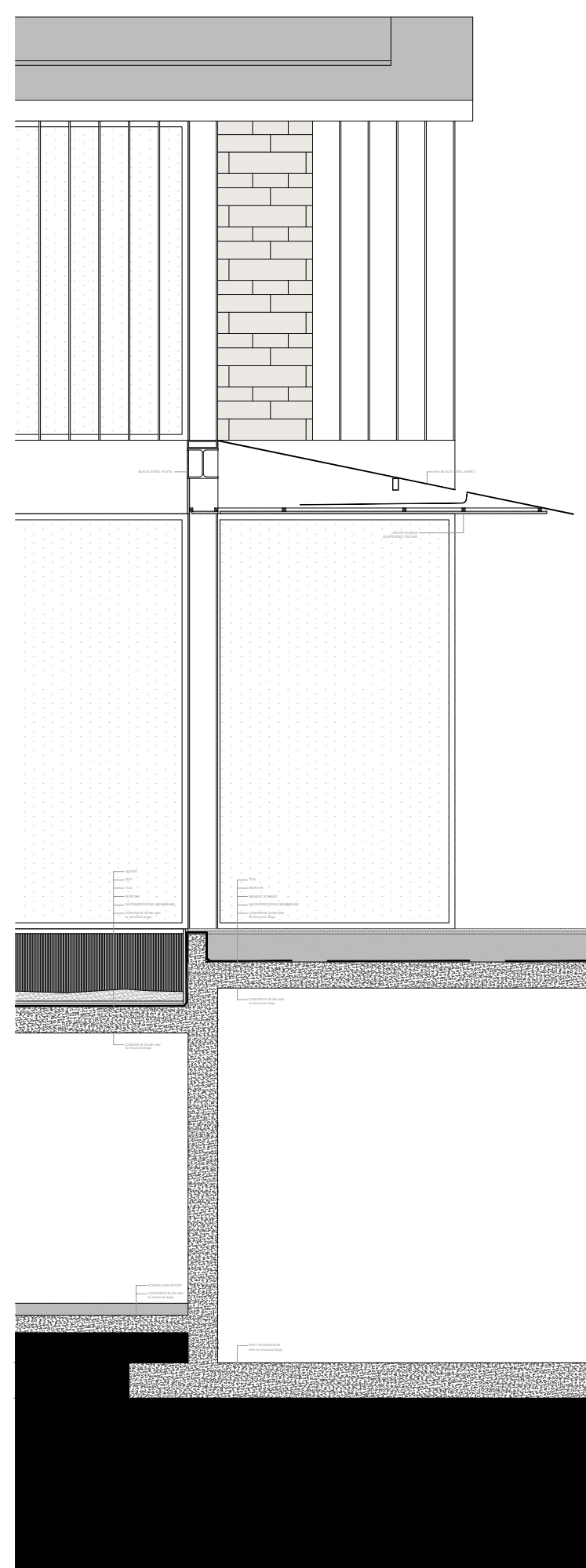
WALL DETAIL B
