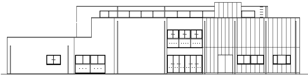
nouth elevation
