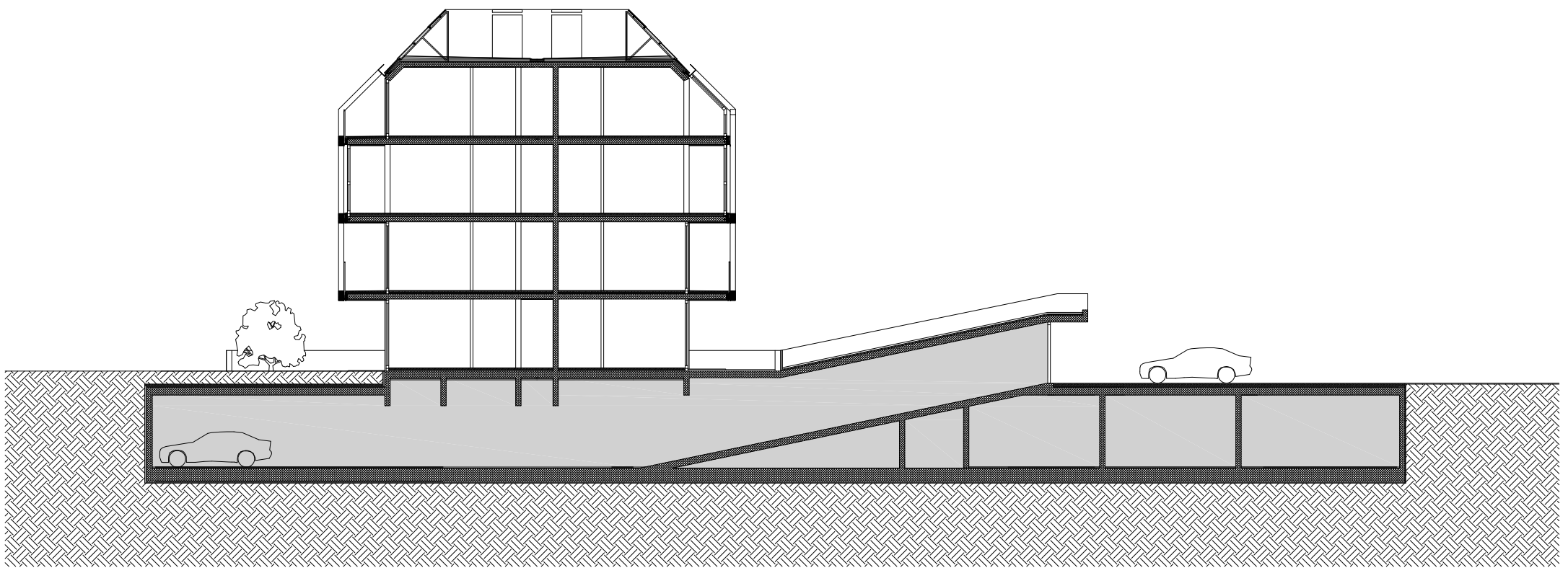
SECTION A
