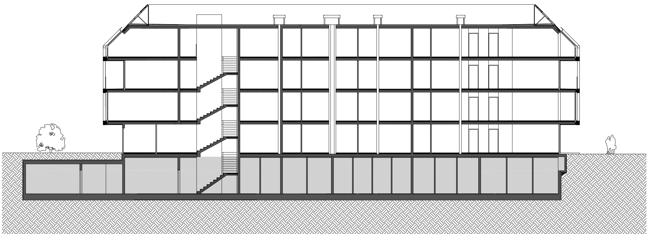
SECTION B
