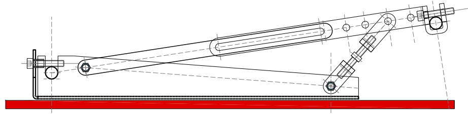
SIDE ELEVATION
