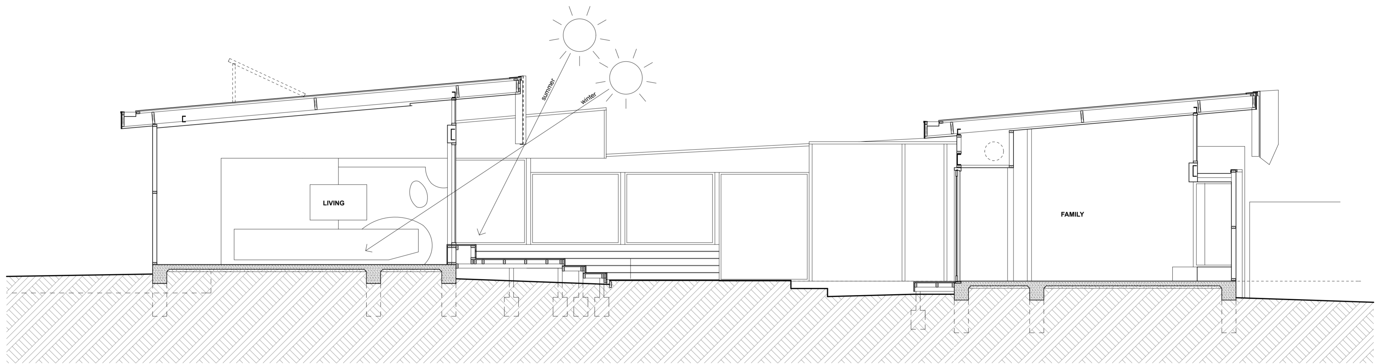
S/11 Section 1:50
