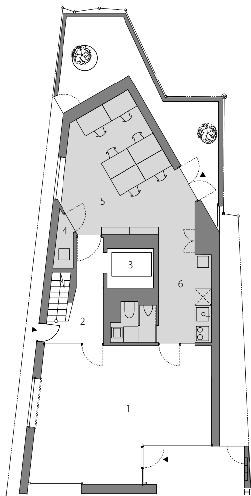
1F PLAN
