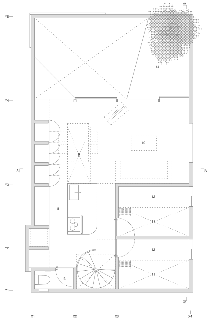
2F plan 1:100
