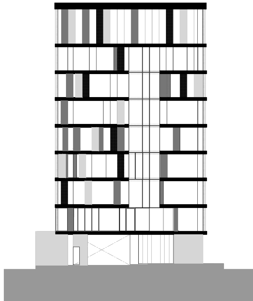
SOUTH ELEVATION 2
