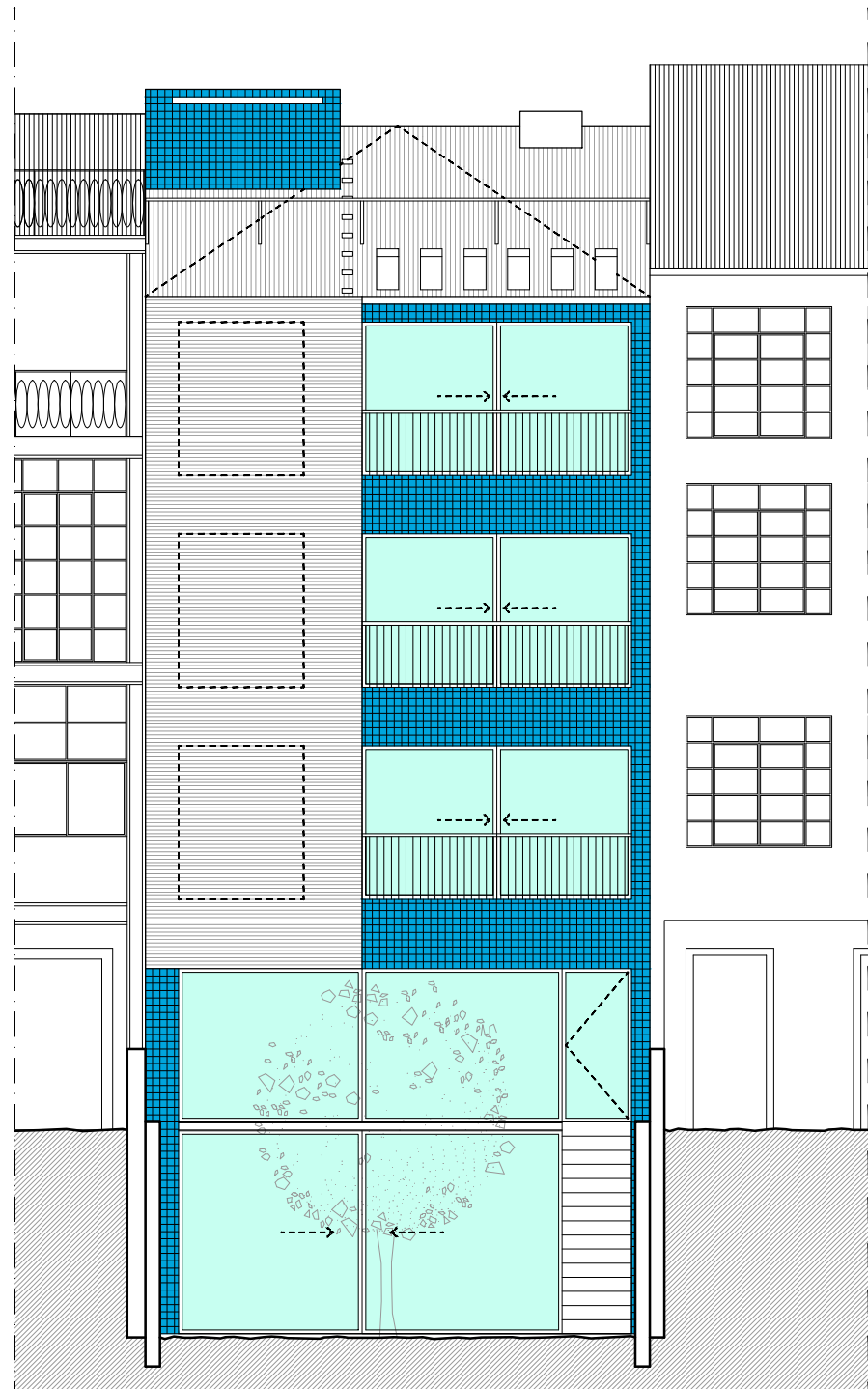
REAR ELEVATION
