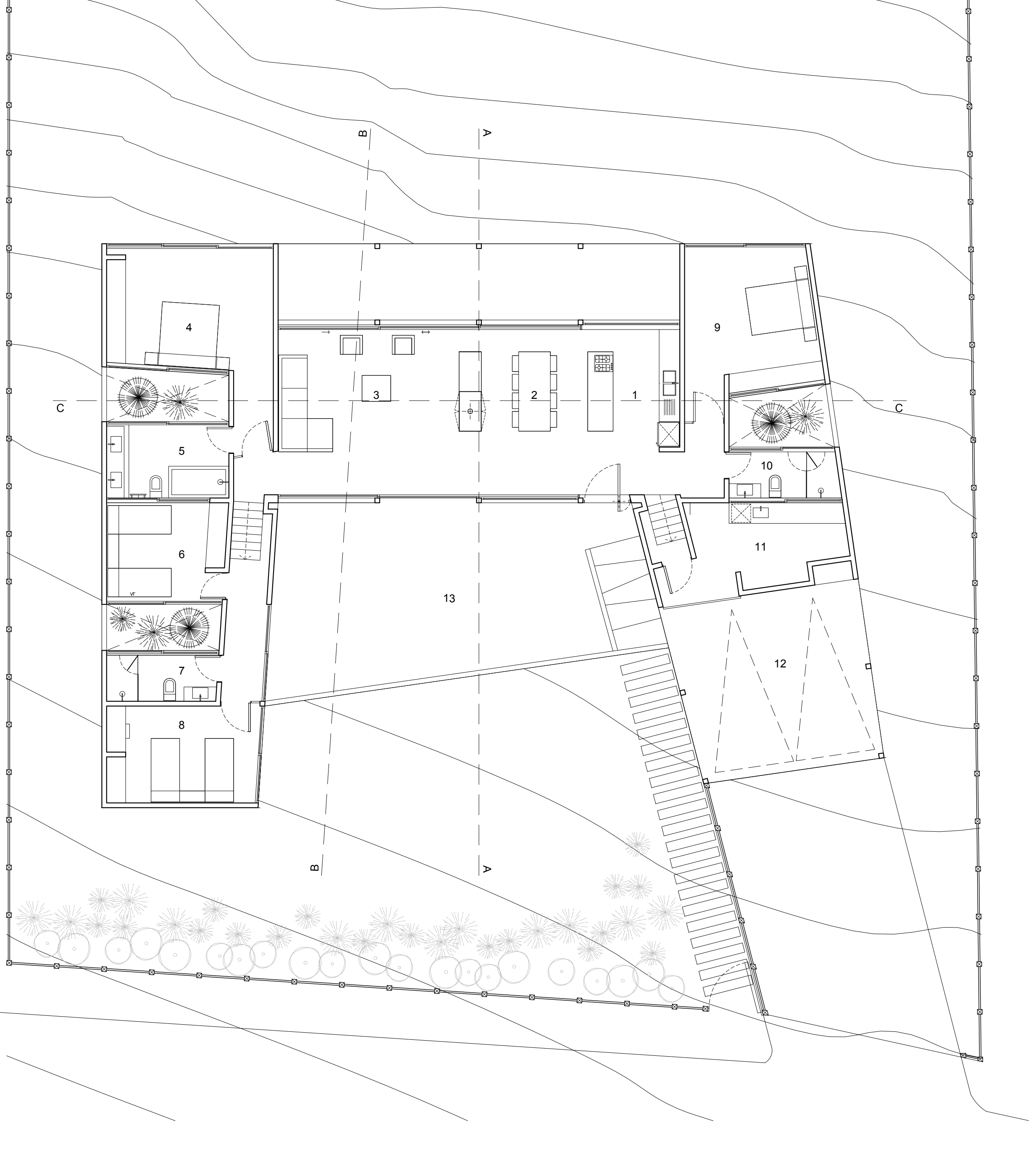
FLOOR PLAN 1.KITCHEN 2.DINING ROOM 3.LIVING ROOM 4.BEDROOM 5.BATHROOM 6.BEDROOM 7.BATHROOM 8.BEDROOM 9.BEDROOM 10.BATHROOM 11.SERVICE YARD 12.PARKING AREA 13.CENTRAL COURTYARD
