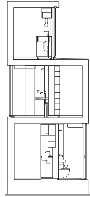
cross section
