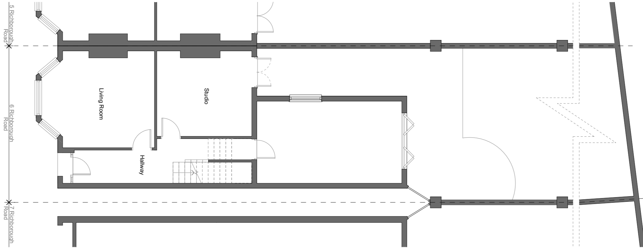
1. Existing Ground Floor Plan
