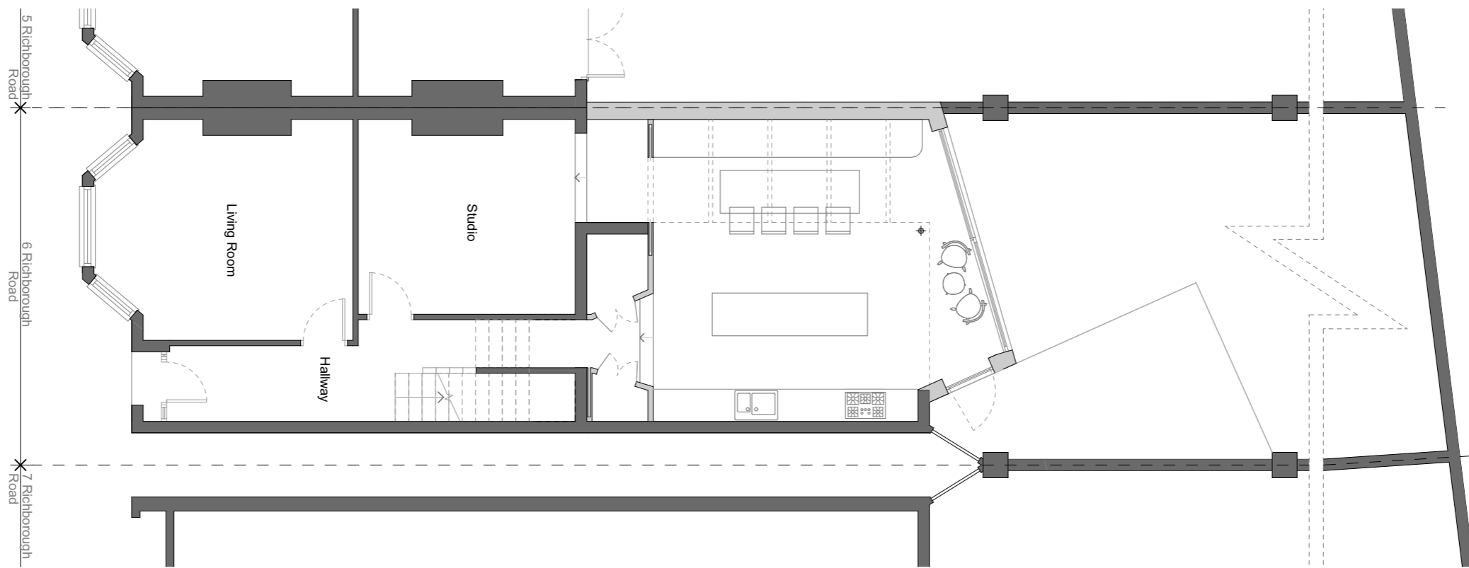
2. Proposed Ground Floor Plan
