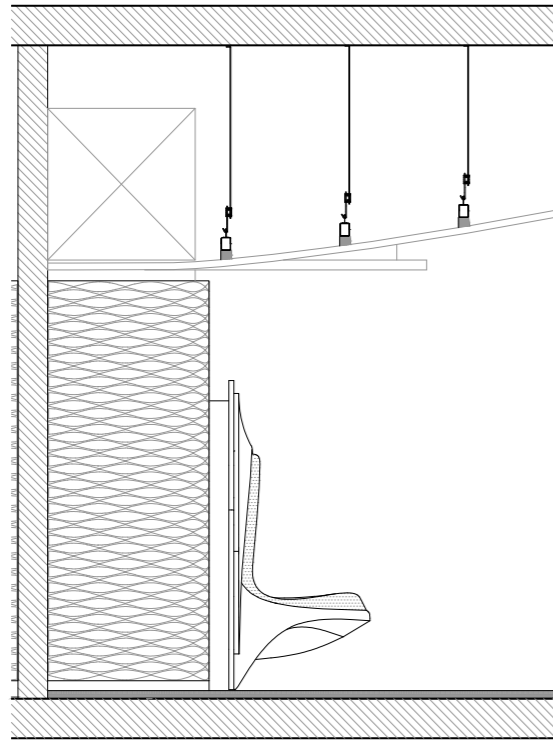
SOFA SIDE ELEVATION
