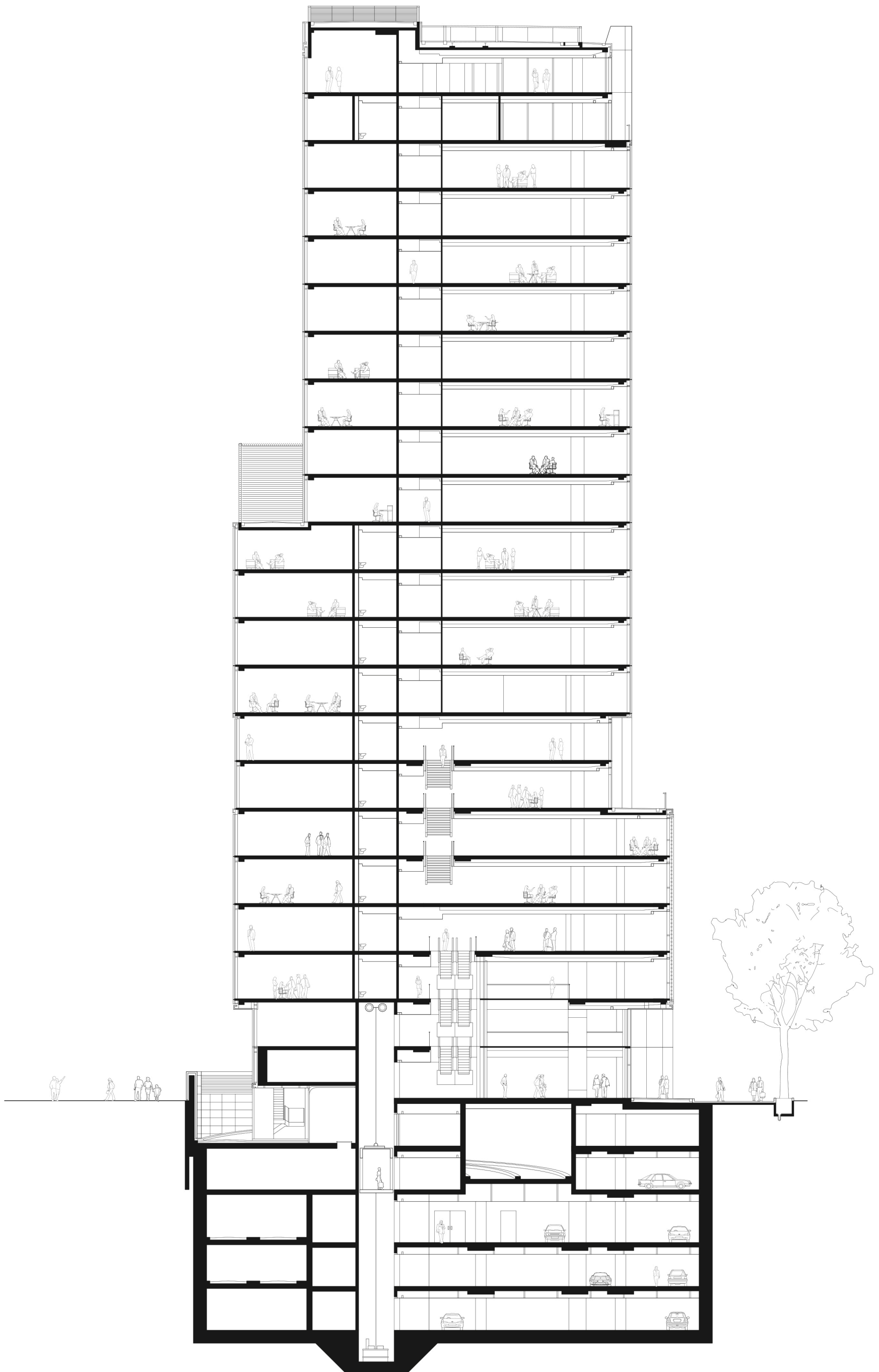
Techcombank Hanoi - Cross Section
