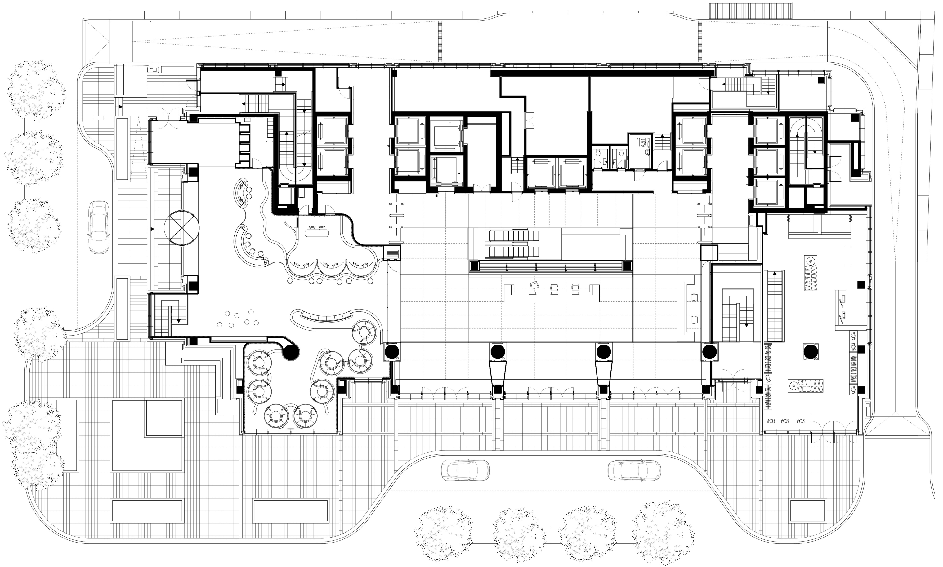
Techcombank Hanoi - Floorplan Groundfloor
