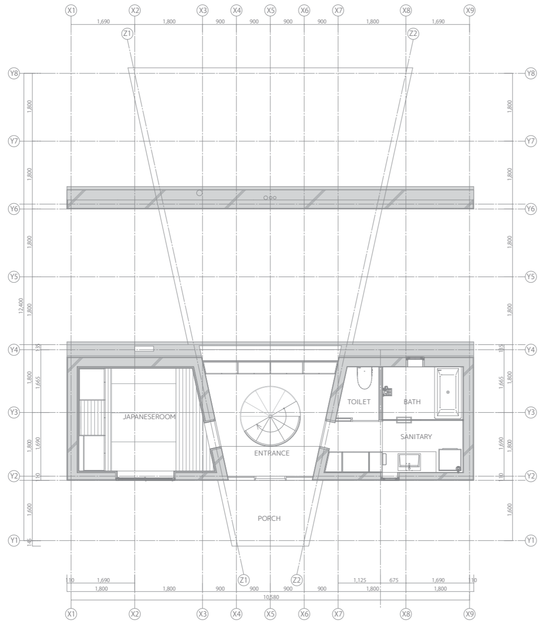
1F PLAN
