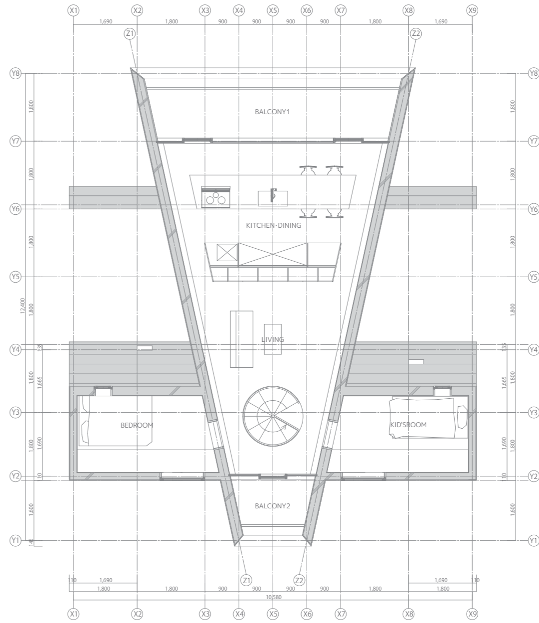
2F PLAN
