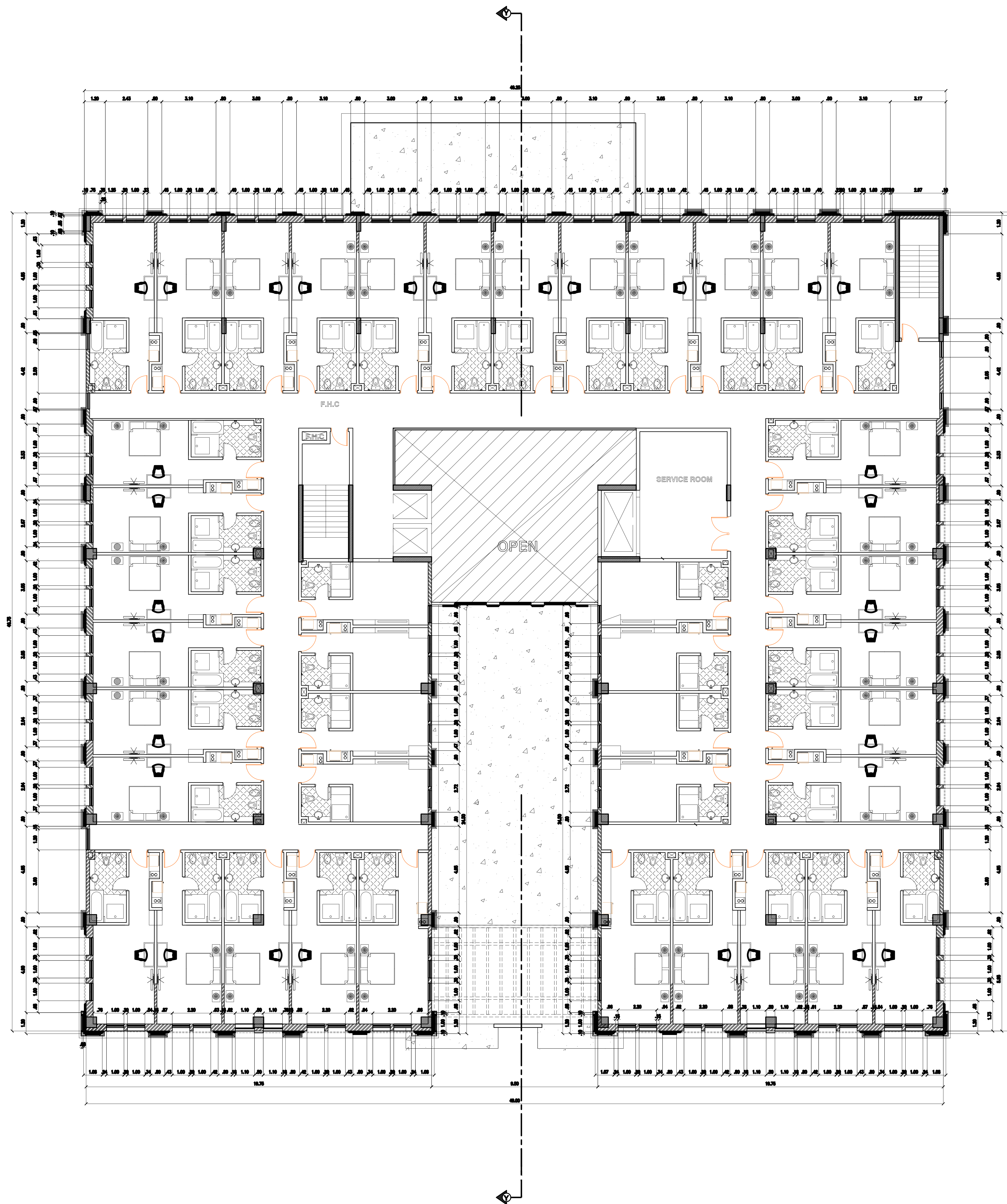
1 A/S SCALE 1:100 M. FIRST FLOOR PLAN BUILDING - B
