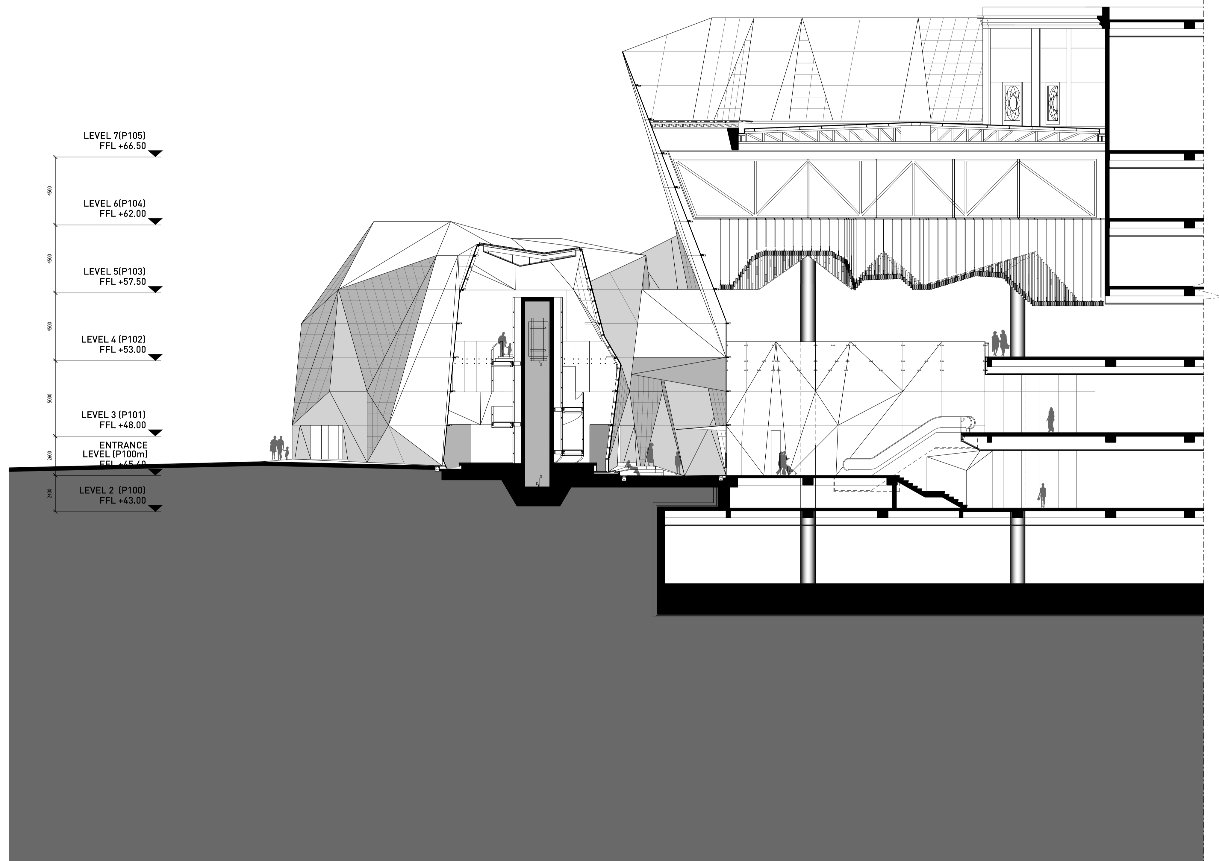
1 SECTION THROUGH GALLERY ATRIUM + PAVILION GA/s205 SCALE 1:150
