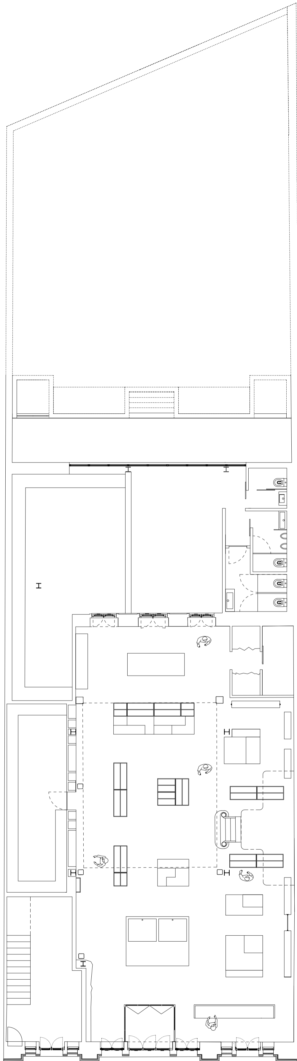
GROUND FLOOR_PLAN_1_100 ESC
