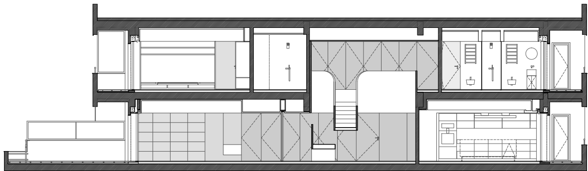
SECTION B
