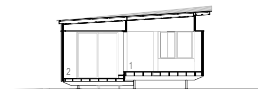
SHORT SECTION
