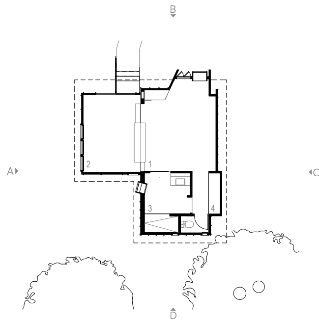
FLOOR PLAN
