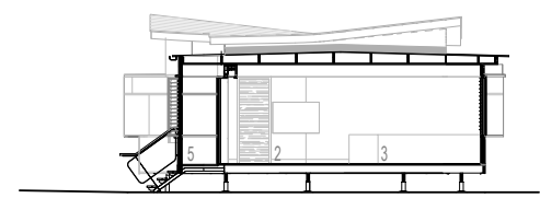
SHORT SECTION
