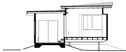
LONG SECTION
