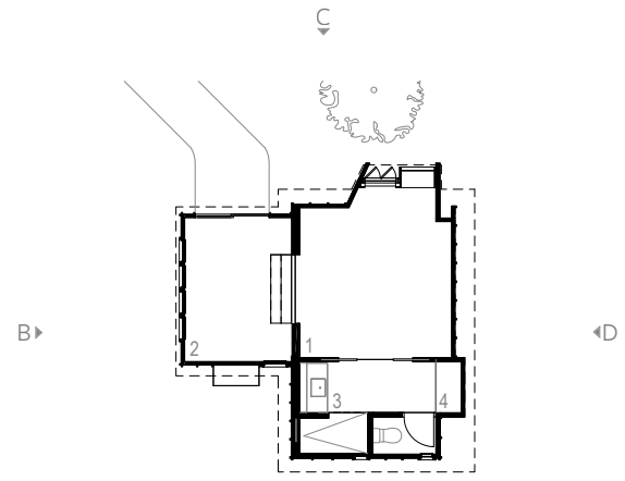
FLOOR PLAN
