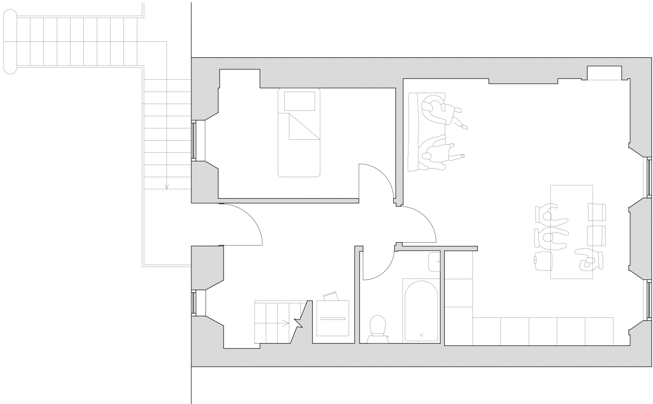
First (Main) Floor Plan
