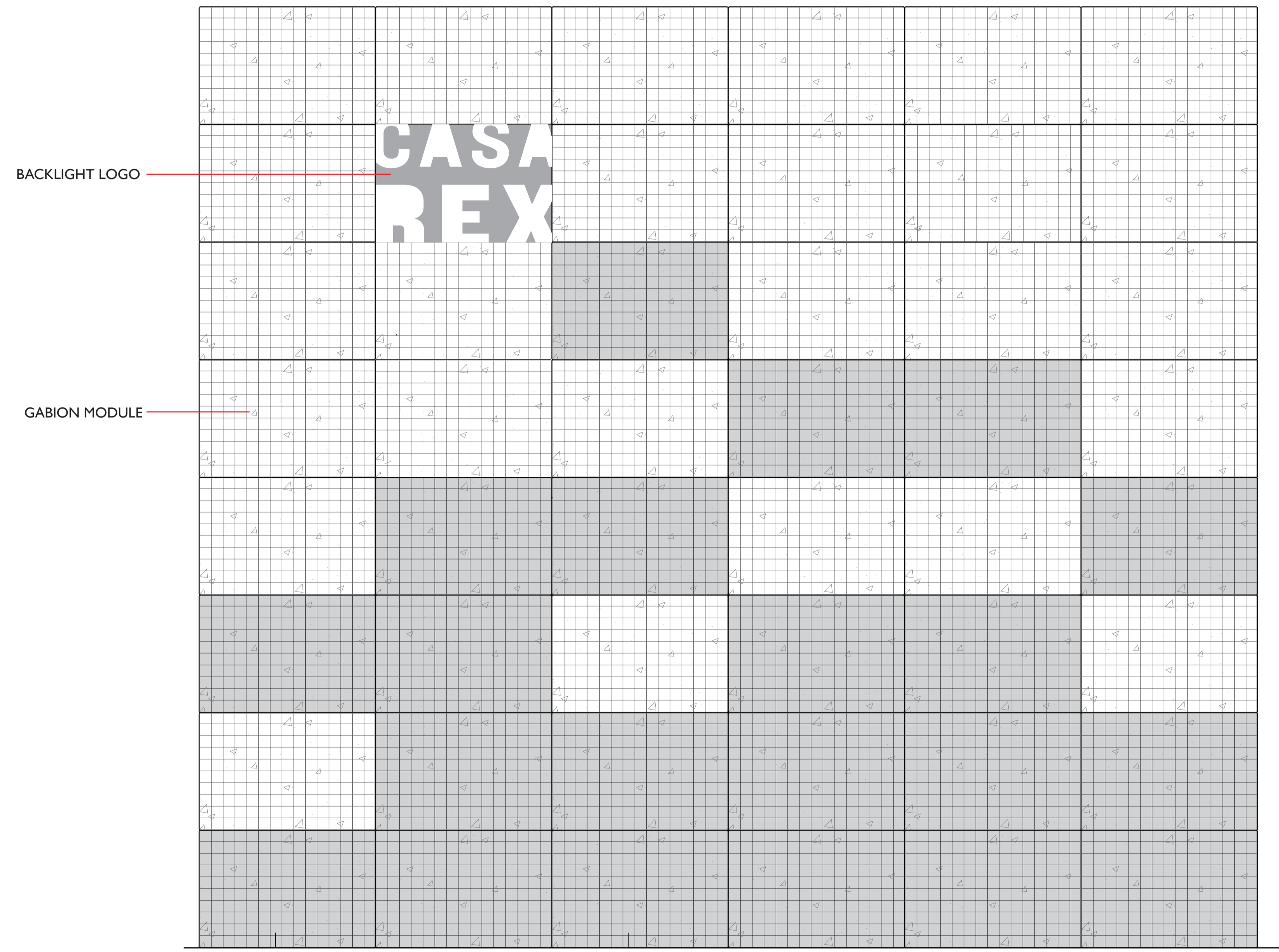
FAÇADE - VIEW 0 0.5 1 2
