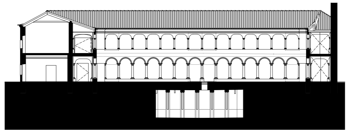
corte 3-3'. section 3-3'
