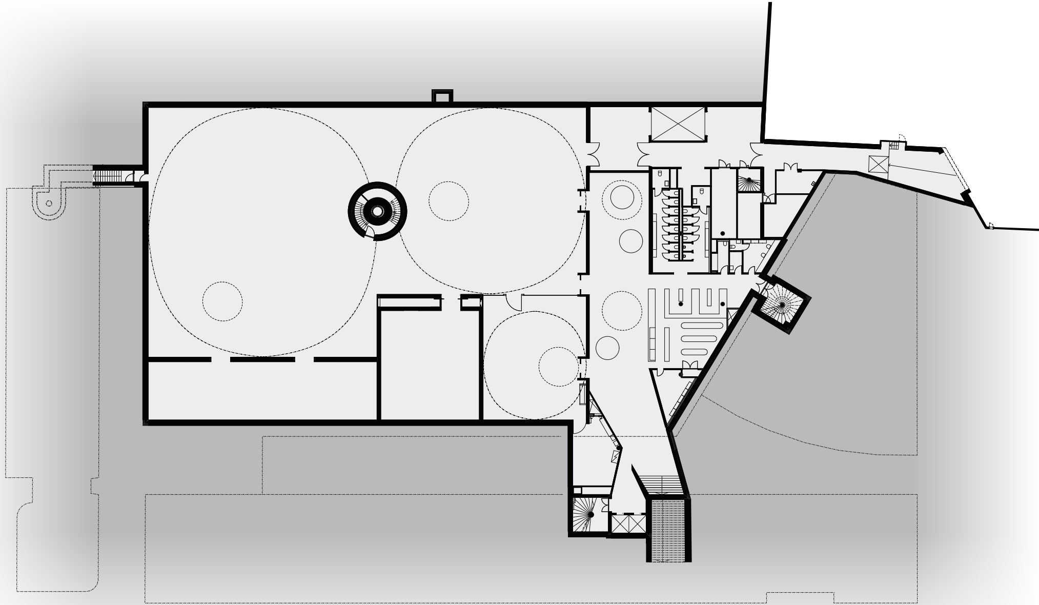
Amos REX -1. Floor 1:500
