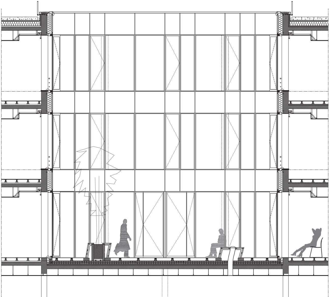
COUPE FACADE TYPE PATIO
