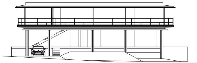
East Elevation
