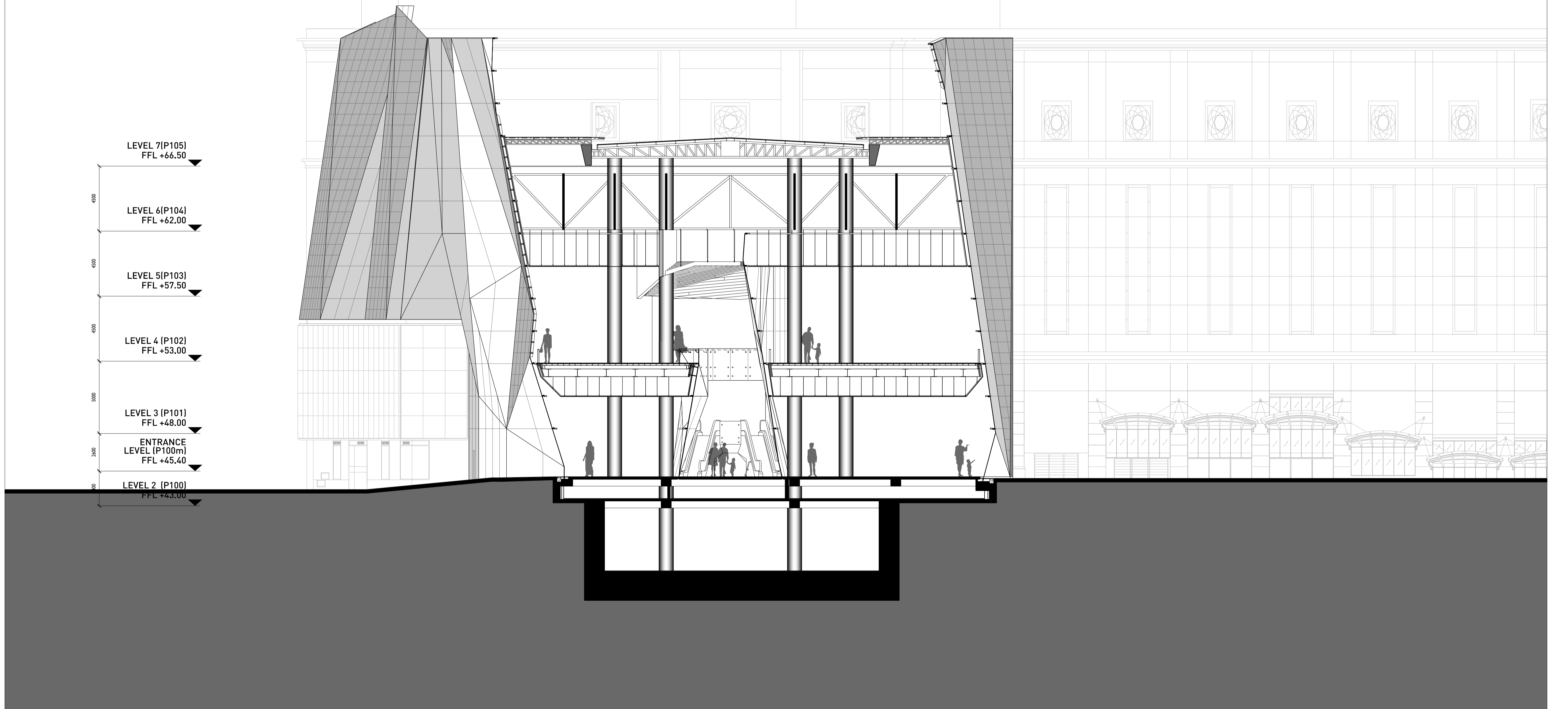
1 SECTION THROUGH ATRIUM GA/s201 SCALE 1:150
