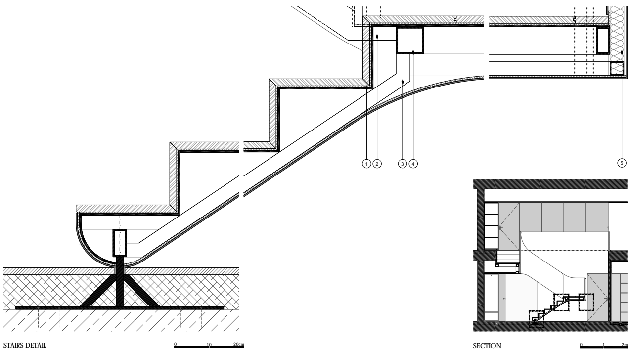
STAIRS DETAIL
