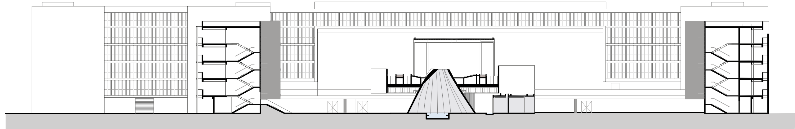
C-C' Section
