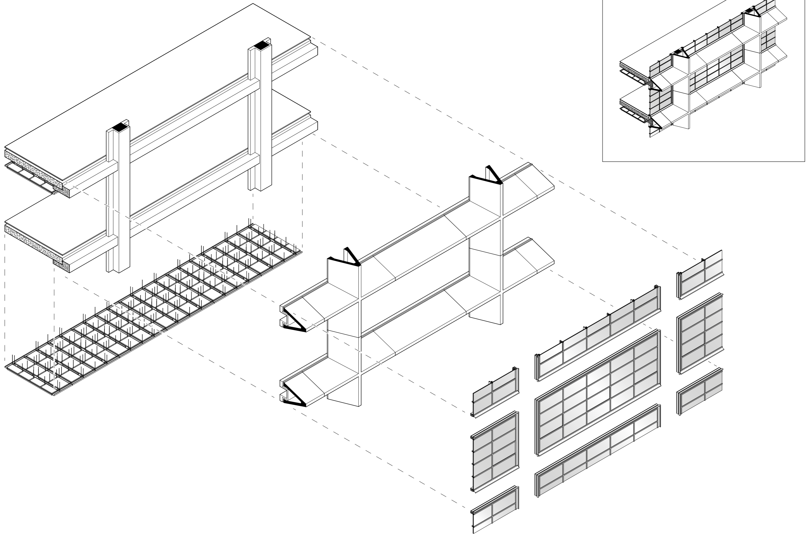
Facade Elements
