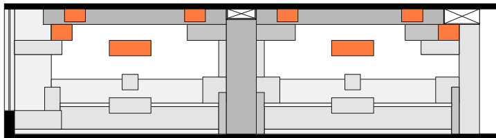
Sextion B, 1:100
