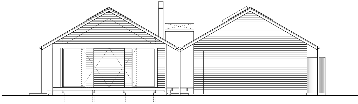
NORTH ELEVATION
