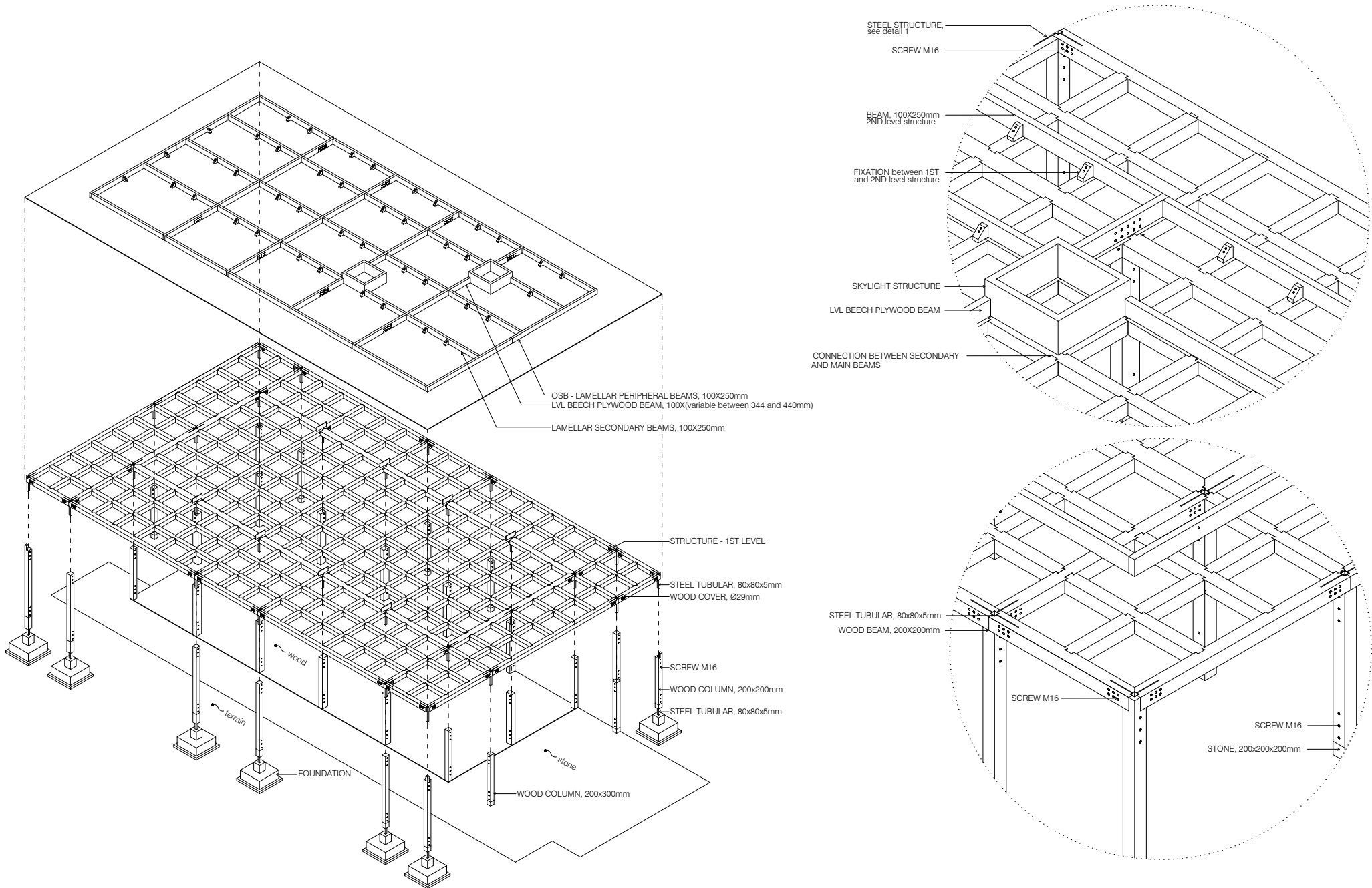
STRUCTURE AXONOMETRIC VIEW
