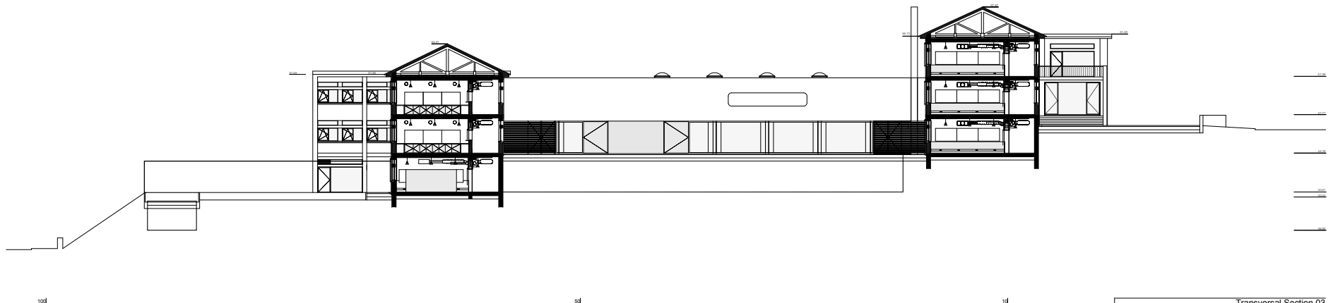
Transversal Section 03
