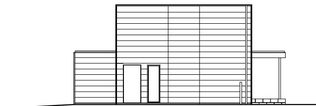
east elevation 1
