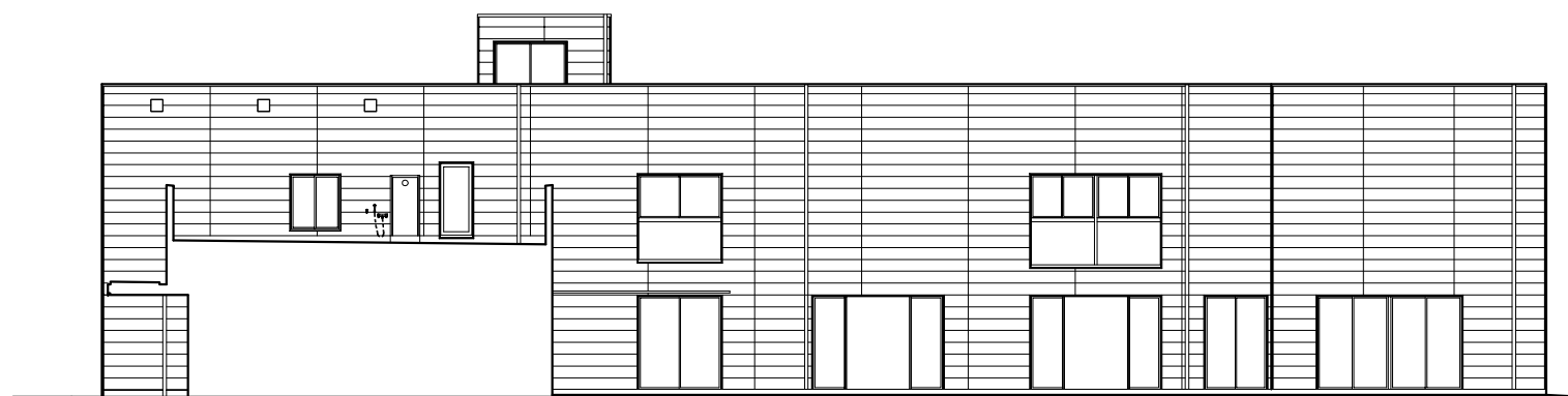
east elevation 2
