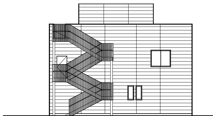
north elevation 1
